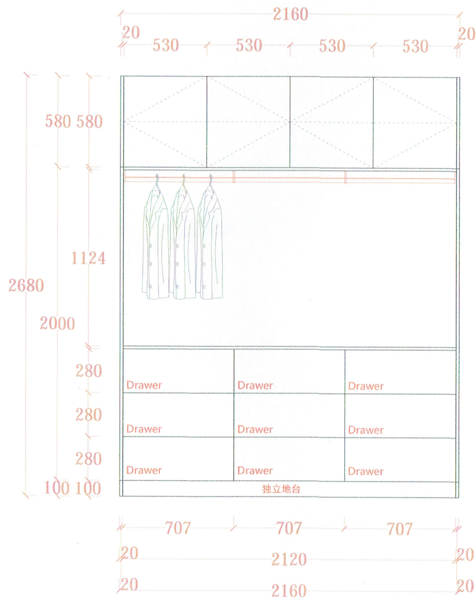
OUTSIDE VIEW A
