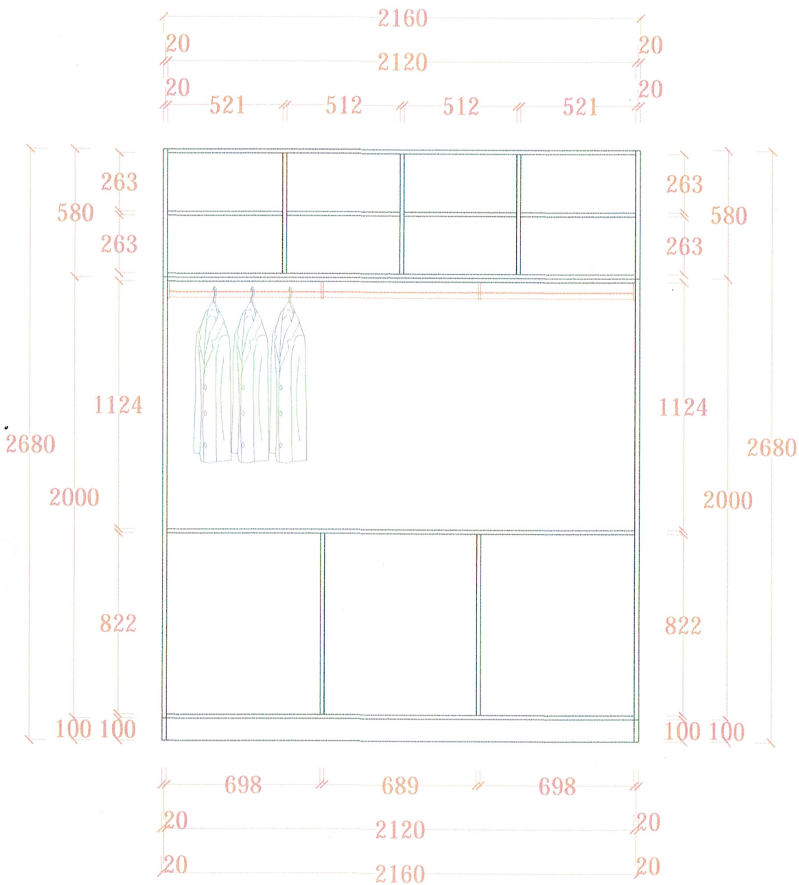
INNER VIEW A
